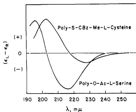
FIGURE 1: Circular dichroism spectra of poly-S-carbobenzoxy-methyl-L-cysteine and poly-O-acetyl-L-serine films.
